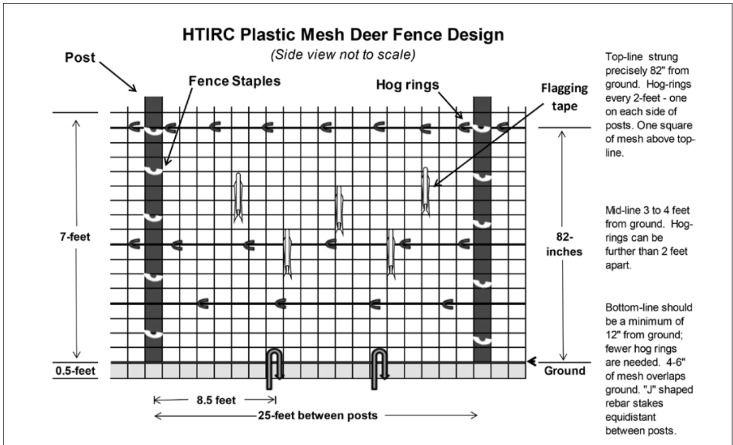
Figure 8. Side view of typical fence construction between posts.
